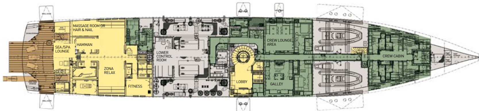
LOWER DECK
